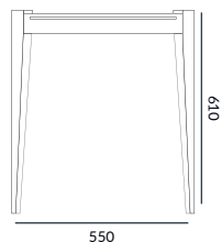
Elevation - without shelf
