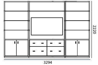
Elevation for single unit
