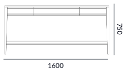
Back elevation - with stretchers
