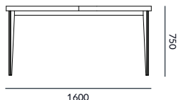
Side elevation
